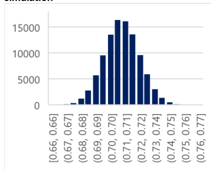
Figure 34 Histogram - Monte Carlo simulation
