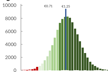
Figure 32: Monte Carlo Simulation
