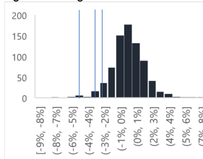
Figure 33 Histogram – Historical method
