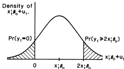
FIGURE 2.—Distribution of y , in censored and "symmetrically censored" sample.
