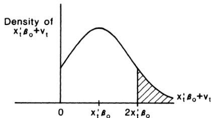
FIGURE 1.—Density function of y_i in truncated and “symmetrically truncated” sample.
